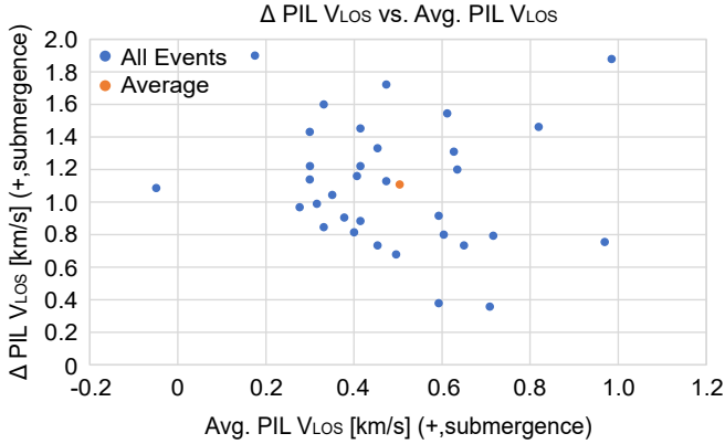
Figure 6. Scatter plot of \Delta V_{\text{LOS}} vs. V_{\text{LOS,avg}} for all events. Recall that \Delta V_{\text{LOS}} is the difference between the extreme values of V_{\text{LOS}} over the lifetime of the event.
