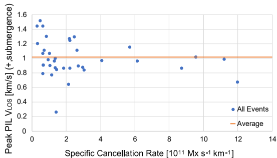
Figure 9. Scatter plot of peak Doppler velocity, V_{\text{LOS,peak}} vs. specific cancellation rate, r for all events. Recall that r measures cancellation per. unit length of the PIL.
