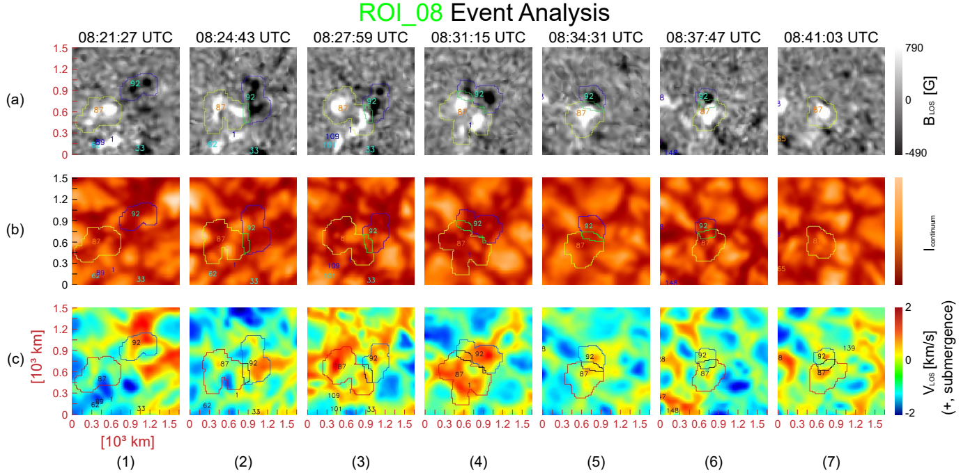
Figure 13. Evolution of B_{\text{LOS}} (top series), 630.1 nm intensity (middle series) and V_{\text{LOS}} (bottom series). ROI_08 in the time series begins with panel 1 (time immediately before PIL is defined) and progresses to panel 7 (time immediately after PIL is no longer defined).
