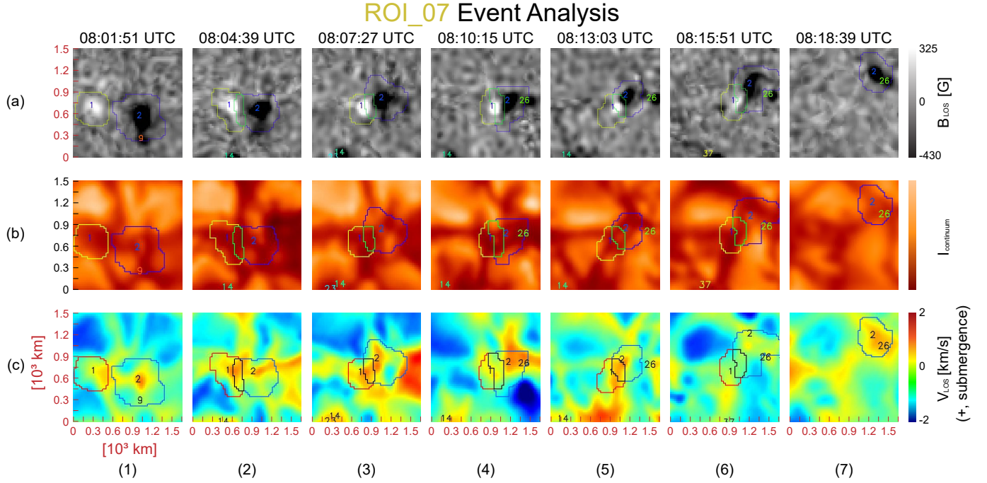
Figure 11. Evolution of B_{\text{LOS}} (top series), 630.1 nm intensity (middle series) and V_{\text{LOS}} (bottom series). ROI.07 in the time series begins with panel 1 (time immediately before PIL is defined) and progresses to panel 7 (time immediately after PIL is no longer defined).
