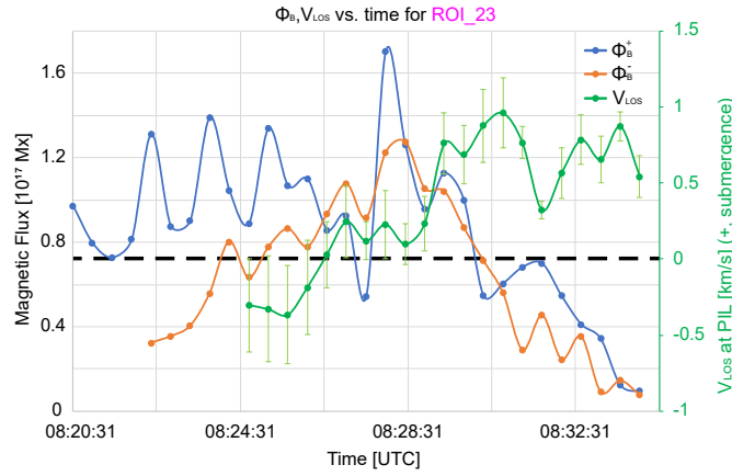
Figure 18. Evolution of LOS magnetic flux and PIL mean Doppler velocity, \Phi_B and V_{LOS} , in ROI_{23} . Refer to the caption of Figure 4 for an explanation of the legend and other graphical details.
