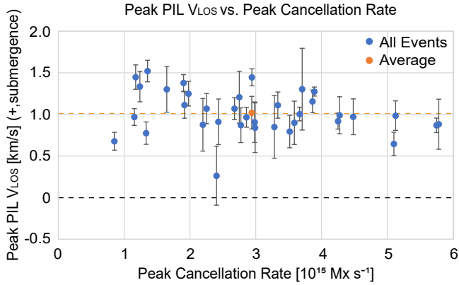
Figure 8. Scatter plot of peak Doppler velocity, V_{\text{LOS,peak}} vs. peak flux cancellation rate, R_{\text{peak}} for all events. Recall that positive values of R_{\text{peak}} indicate flux cancellation while negative values indicate flux accumulation.
