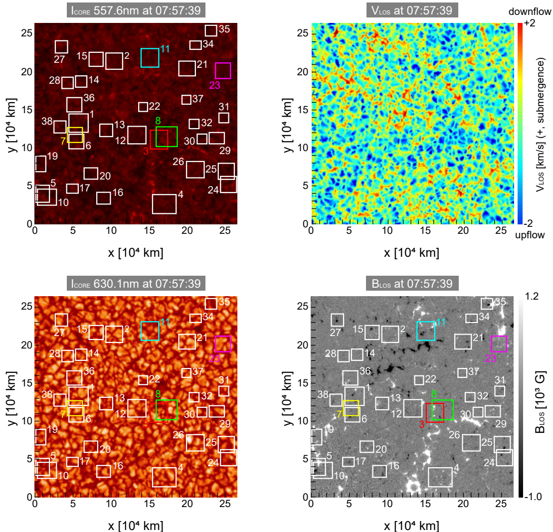
Figure 1. Four snapshot views of a quiet Sun region at the disk center, as observed by the SST. Top left: Core intensity in the non-magnetic Fe I 557.6 nm line. Top right: Line-of-sight velocity ( V_{\text{LOS}} ) with positive and negative values corresponding to downflows and upflows, respectively. Bottom left: Continuum image at Fe I 630.1 nm. Bottom right: Line-of-sight magnetogram ( B_{\text{LOS}} ). Rectangles indicate analyzed regions of interest (ROI), numbered by the ROI indices. Colored rectangles are events described in section 4.1 and A of the manuscript.
