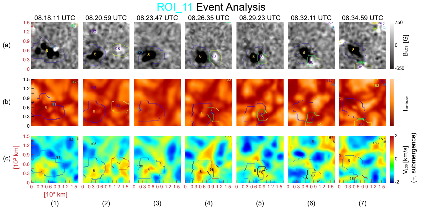
Figure 15. Evolution of B_{LOS} (top series), 630.1 nm intensity (middle series) and V_{LOS} (bottom series). ROI_{11} in the time series begins with panel 1 (time immediately before PIL is defined) and progresses to panel 7 (time immediately after PIL is no longer defined).
