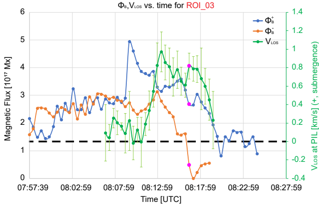
Figure 4. Evolution of LOS magnetic flux \Phi_B and PIL mean Doppler velocity V_{\text{LOS}} in ROI 03 . Blue data points are \Phi_B^+ ; orange points are \Phi_B^- . The pink dots represent the time when maximum flux cancellation was achieved. The green data points are V_{\text{LOS}} , and are only counted while the PIL is defined. Positive values of V_{\text{LOS}} represent submergence. A dotted line is placed at V_{\text{LOS}} = 0 \text{ km s}^{-1} to aid in viewing the diagram.
