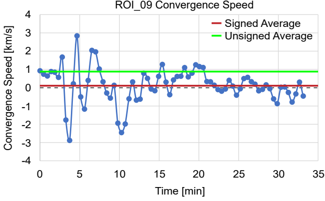
Figure 5. Convergence speed, v_{\text{conv}} , over the cancellation duration as calculated with the COG method for ROI.09. As the cancelling features occasionally drift apart, the v_{\text{conv}} becomes negative. The average v_{\text{conv}} for that event, 0.1 \text{ km s}^{-1} is represented by the red line. The proper motion speeds are calculated by v_{\text{proper}} = |v_{\text{conv}}| , and the mean value is shown by the green line, which is 0.7 \text{ km s}^{-1} . ROI.09 is shown here since it exhibits strong polarity drift.
