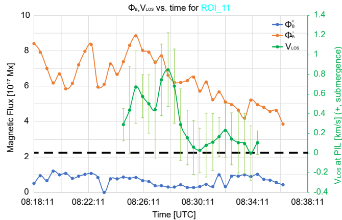
Figure 16. Evolution of LOS magnetic flux and PIL mean Doppler velocity, \Phi_B and V_{LOS} , in ROI_{11} . Refer to the caption of Figure 4 for an explanation of the legend and other graphical details.
