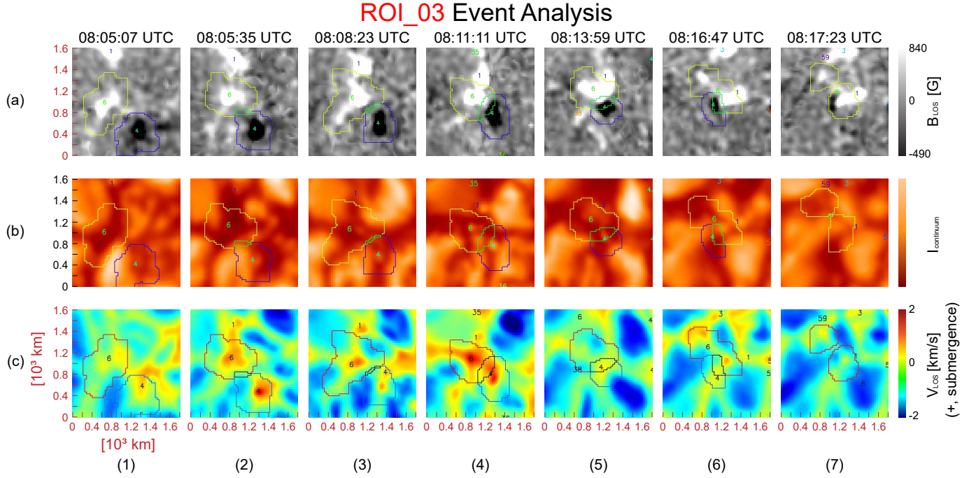
Figure 3. Evolution of B_{\text{LOS}} (top series), 630.1 nm intensity (middle series) and V_{\text{LOS}} (bottom series). ROI 03 in the time series begins with panel 1 (time immediately before PIL is defined) and progresses to panel 7 (time immediately after PIL is no longer defined).
