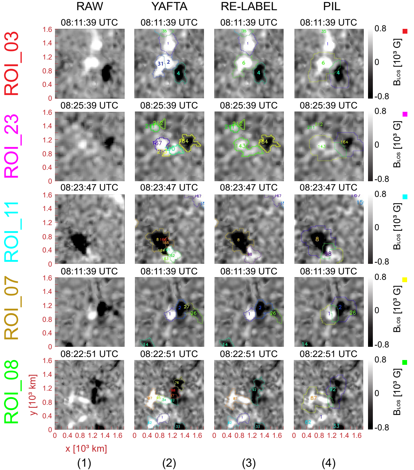
Figure 2. B_{\text{LOS}} time snapshots of 5 distinct cancellations showing the different steps of processing with YAFTA, as described in Section 2. Column (1) shows the raw magnetogram image of the ROI. Column (2) shows the initial tracking result with YAFTA. Column (3) shows the re-labeled features. Column (4) shows the two cancelling features, their dilated masks, and PIL (green outline). Each row of images represents a different ROI. The color of the square beside the right-most image corresponds to the color of the ROI in the full field of view magnetogram in Figure 1.
