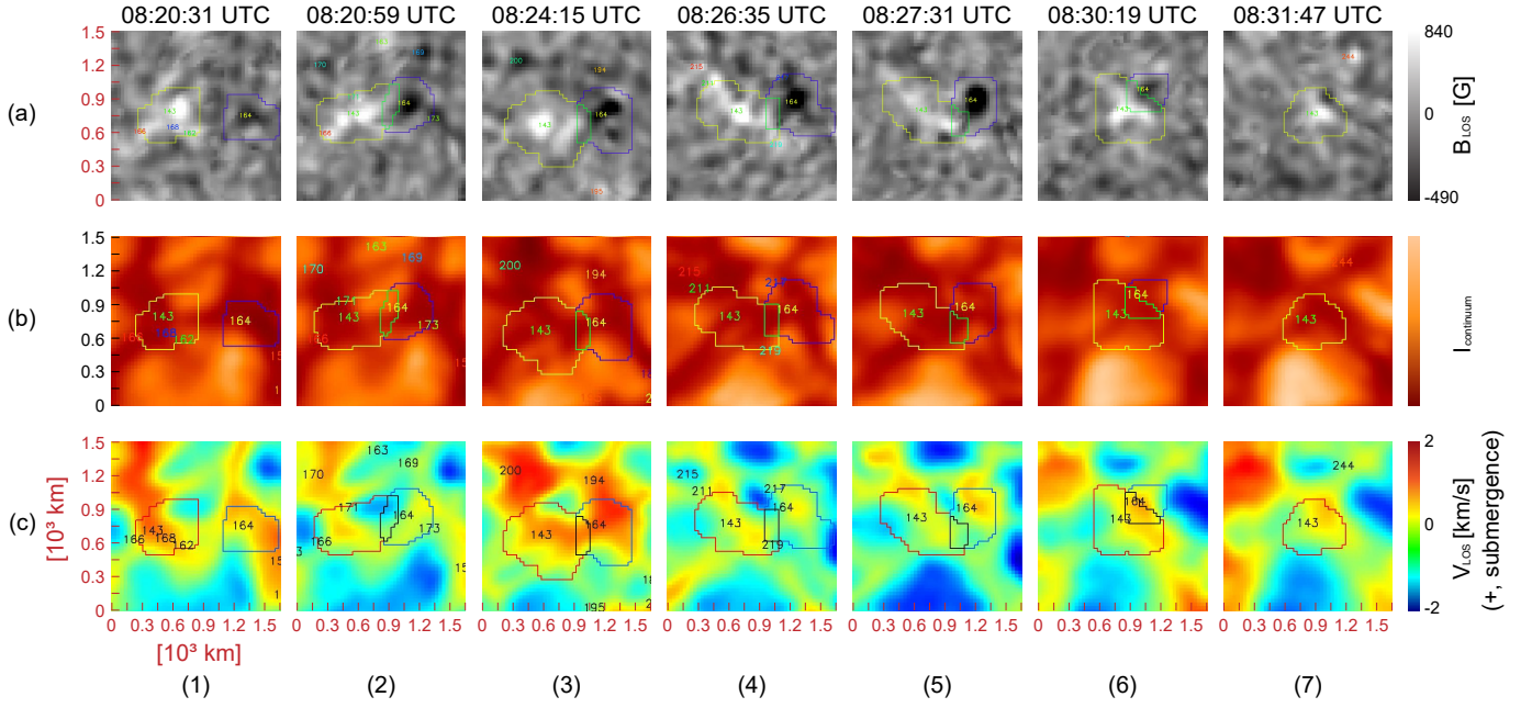
Figure 17. Evolution of B_{LOS} (top series), 630.1 nm line core (middle series) and V_{LOS} (bottom series). ROI_{23} in the time series begins with panel 1 (time immediately before PIL is defined) and progresses to panel 7 (time immediately after PIL is no longer defined).
